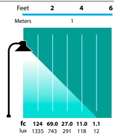
PL-16 Half Spread Photometrics 10 ft. (3.0m) diameter
